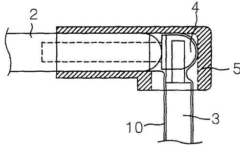
FIG. 1 CONVENTIONAL ART
